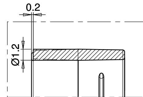
gate detail scale 4:1
