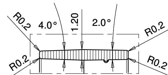
section C-C scale 4:1
